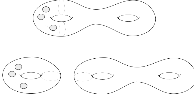
Figure 6: The surfaces G_r and F_r \sqcup \Sigma_2 , used in constructing Z_0 and Z'_0 respectively.
