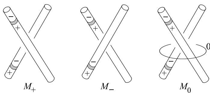
Figure 3: Sutured manifolds obtained from the knot complement, related by a surgery exact triangle.
