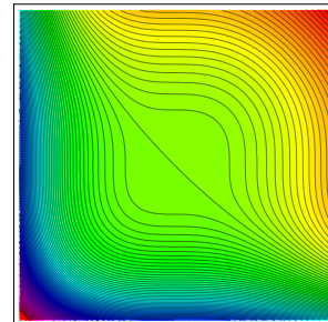
The picture shows contour lines of g(x, y)
