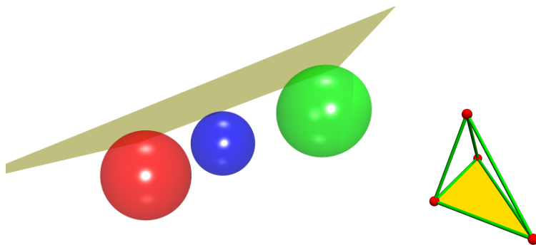
FIGURE 2. The sphere problem and the tetrahedron.
