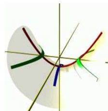
HYPERBOLIC PARABOLOID
