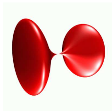
QUARTIC
