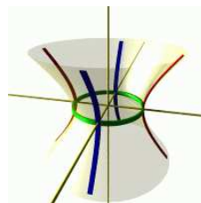
HYPERBOLOID I
