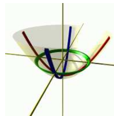
PARABOLID
