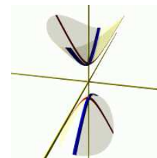
DEFORMED HYPERBOLOID
