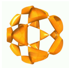
SEXTIC
