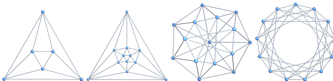
FIGURE 1. The octahedron has K(v) = 1/3 for all v . The icosahedron has K(v) = 1/6 for all v . A projective plane has curvatures in \{0, 1/6, -1/6\} . The flat torus = Clifford torus has constant curvature 0.
