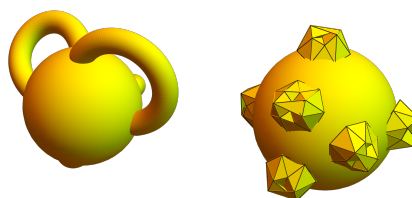
FIGURE 2. A 2-manifold is either S^2 with g handles (orientable) and \chi = 2 - 2g or a S^2 with g cross caps and \chi = 2 - g (non-orientable).
