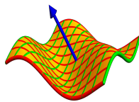
FIGURE 1. A parametrized surface r(u, v) with unit normal vector n(u, v) . When seen as a map from M to S^2 it is known as the Gauss map .
