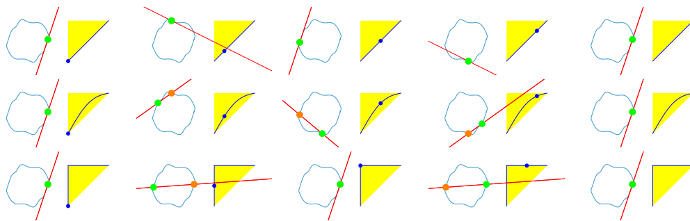
FIGURE 2. The deformation argument.
