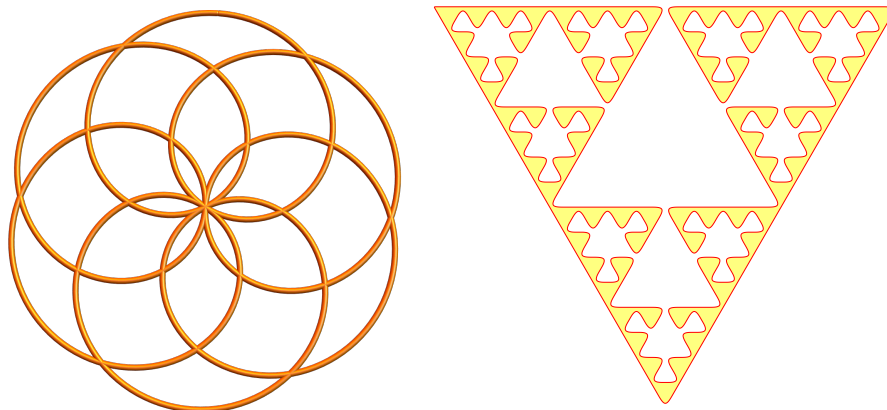
FIGURE 1. To the left, we see r(t) = [\cos(t) + \cos(7t), \sin(t) + \sin(7t)] , t \in [0, 2\pi] which looks like the flower of life. Its rotation number is 7. We can compute \kappa(t)|r'(t)| = 4 + 72/(25 + 8\cos(6t)) which integrates on [0, 2\pi] up to 14\pi . To the right, a simple closed smooth curve in the plane. What is its rotation number?
