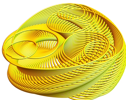
FIGURE 1. An example of a curve with \kappa(t) = a + b \cos(ct), \tau(t) = d \sin(et) .
