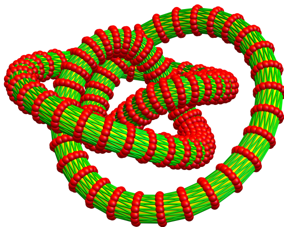
FIGURE 1. A picture of a knot. Drawing the curve in such a fancy way, needs concepts like curvature and torsion, which we will learn next week. The first fundamental form of the figure 8 knot is r'(t)^2 = 101/2 + 36 \cos(2t) + (5/2) \cos(4t) + 8 \cos(8t) . The action is I = 101\pi , the arc length involves elliptic integrals. Numerically it is L = 42.966 \dots . It is typical that we can explicitly give the action but not the length.
