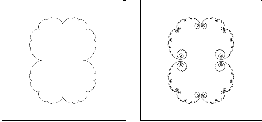
Figure 9. Parabolic implosion.
