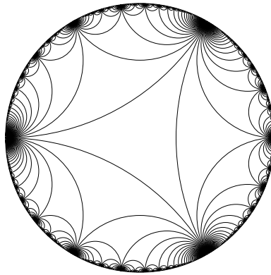
Figure 1. Tiling of the hyperbolic plane by ideal triangles.
