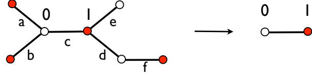
Figure 3. This Belyi tree corresponds to \sigma_0 = (abc)(df) , \sigma_1 = (cde) .
