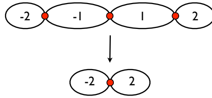
Figure 2. Topology of a cubic polynomial.
