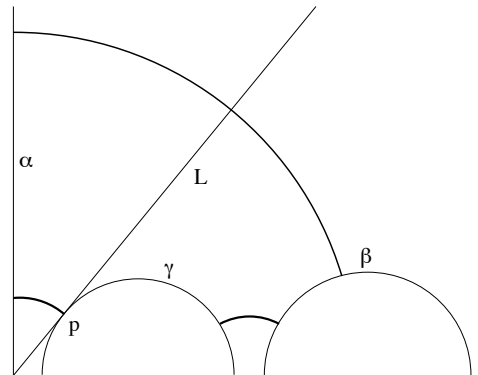
Figure 6. Right hexagons.
