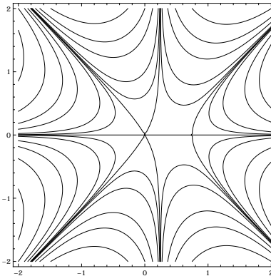
Figure 5. Foliation of df , f(z) = z^3(z - 1) .
