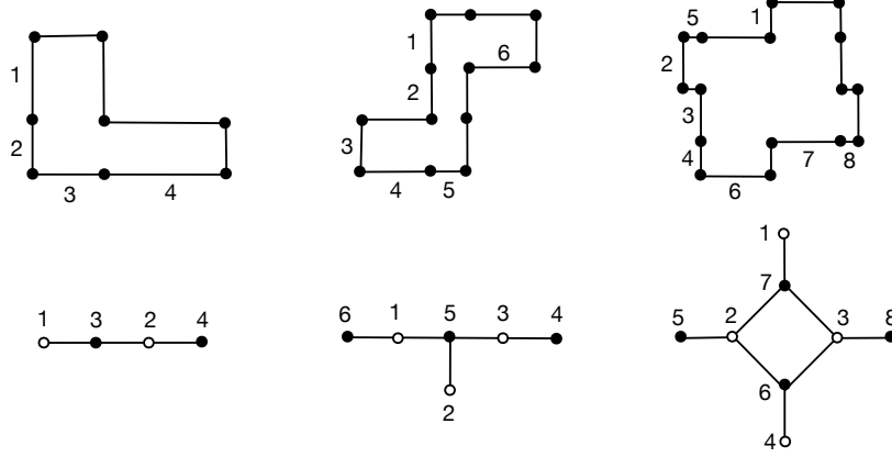
Figure 6.3. Polygons of shapes L, S and X yields surfaces of genus 2, 3 and 4.
