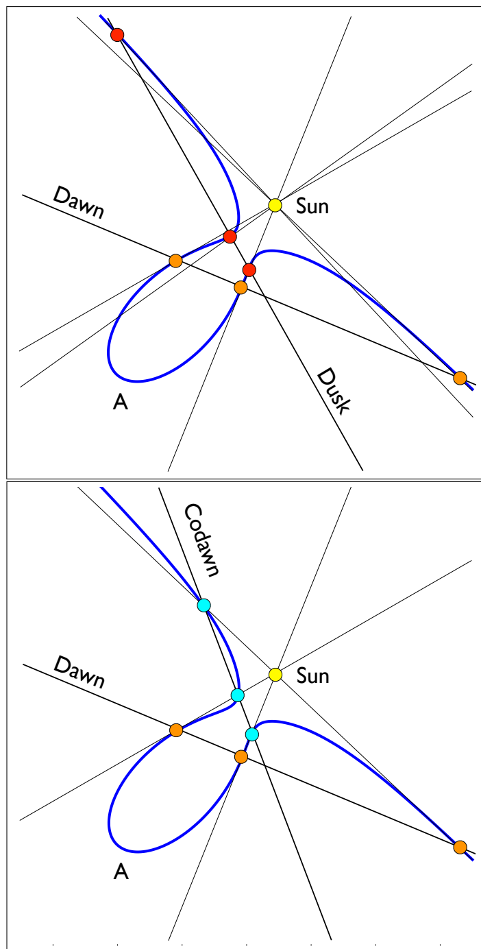
Figure 8.3. The solar configuration.
