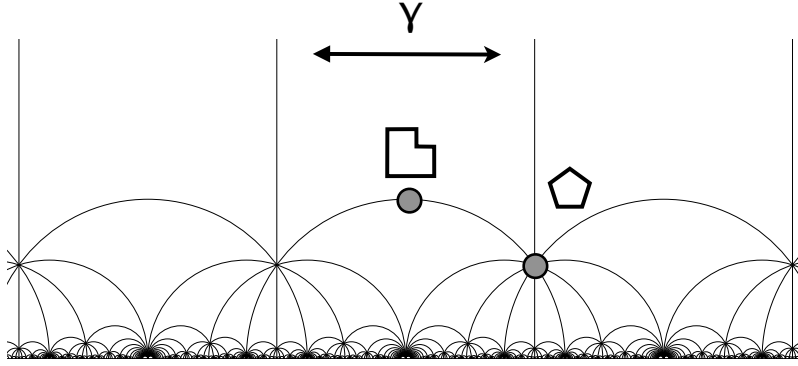
Figure 3.6. The Teichmüller curve f : V = \mathbb{H}/\Delta(2, 5, \infty) \rightarrow \mathcal{M}_2 generated by the golden L and the regular pentagon P .
