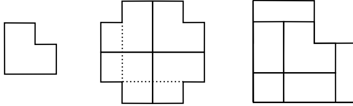
Figure 3.4. Unfolding an L-shaped polygon.
