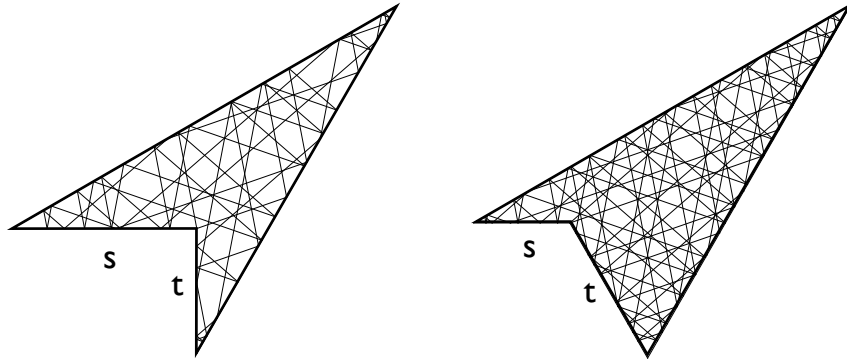
Figure 9.2. Closed billiard paths in Q_{1119}(s, t) and Q_{1128}(s, t) .
