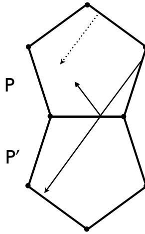
Figure 3.3. The double pentagon P \cup P' yields a surface of genus 2.
