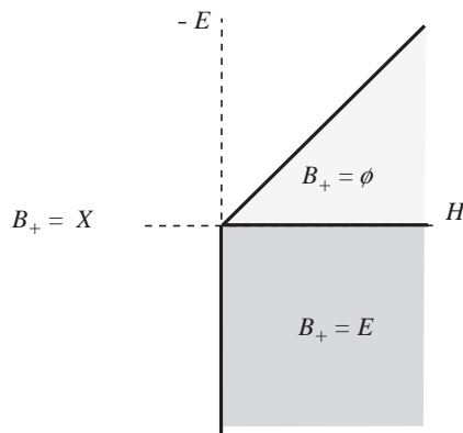
FIGURE 1. Stable classes on blow-up of \mathbf{P}^n
